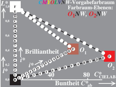
BG091-1, Brilliantheit i^* von O_1, O_2 in (C^*_{ab}, L^*)
