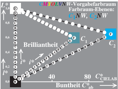
BG091-8, Brilliance i^* von C_1, C_2 in (C_{ab}^*, L^*)
