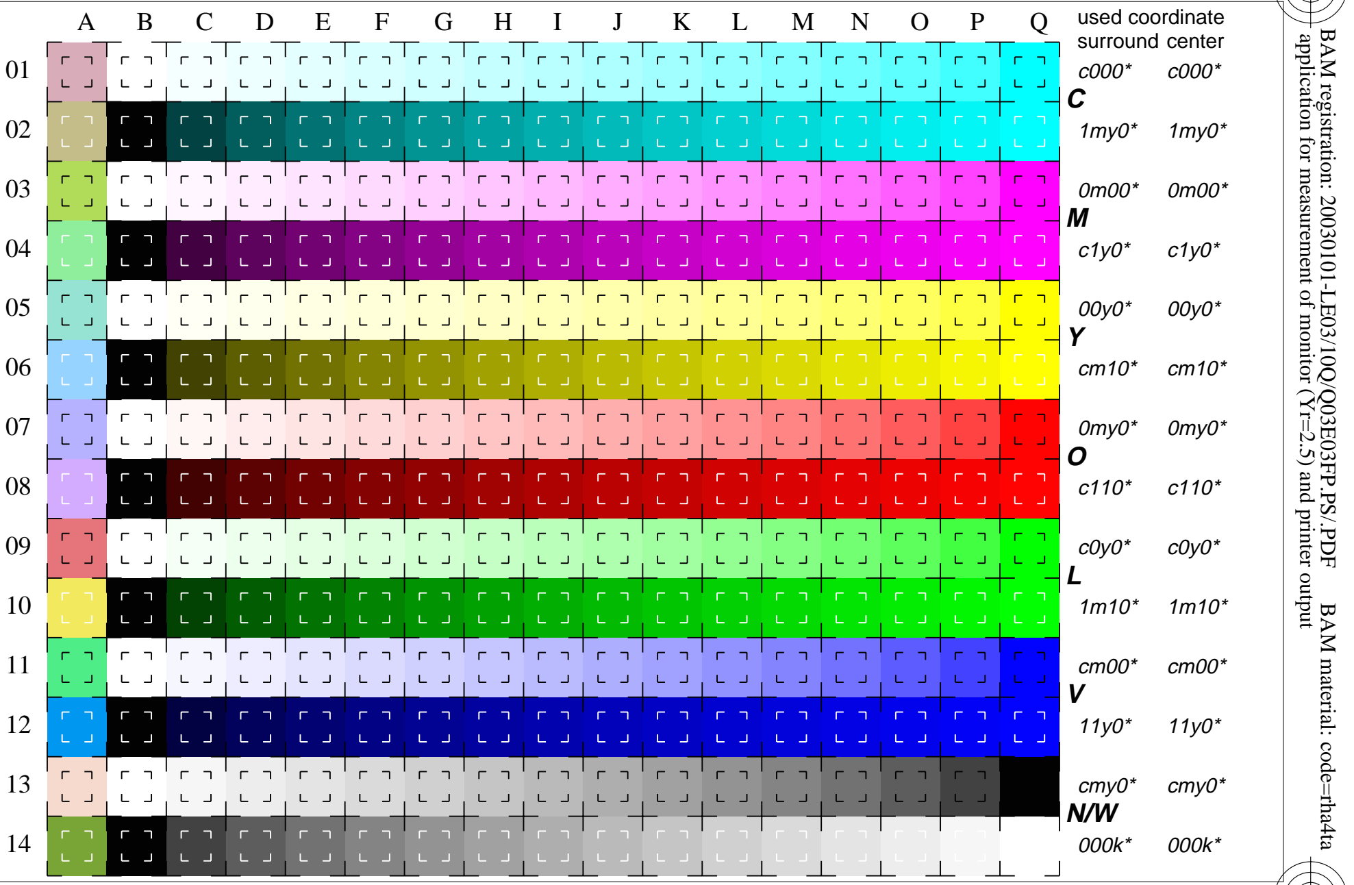
16 equidistant CIELAB steps: C-W, C-N, M-W, M-N, Y-W, Y-N, O-W, O-N, L-W, L-N, V-W, V-N, N-W, W-N and 14 CIE-test colours (left)
