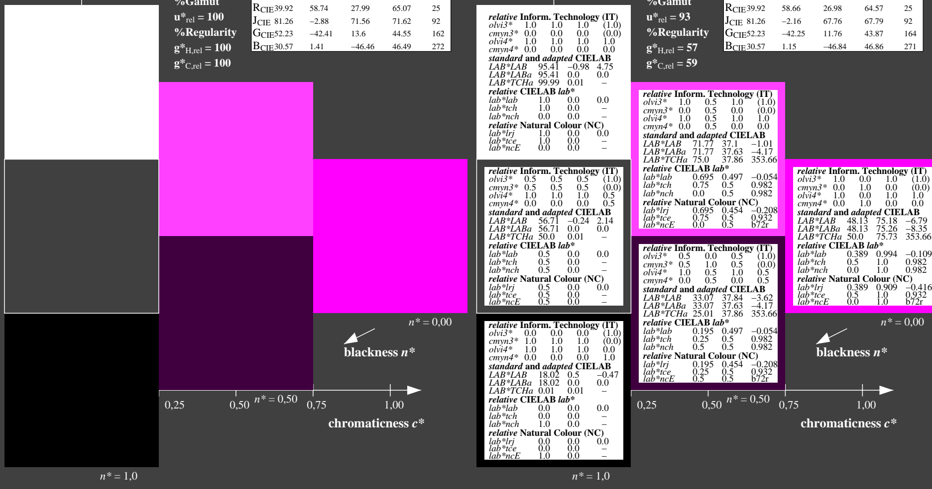
3 step scales for constant CIELAB hue 354/360 = 0.982 (right)
