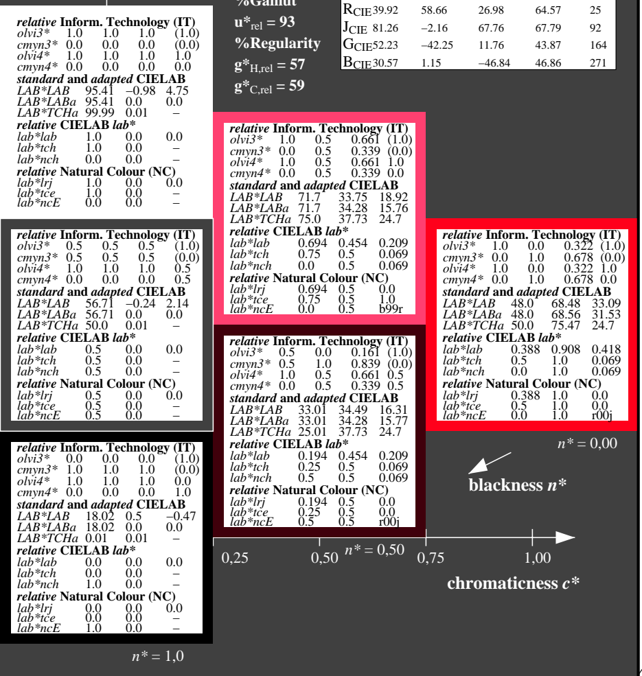
3 step scales for constant CIELAB hue 25/360 = 0.069 (right)
