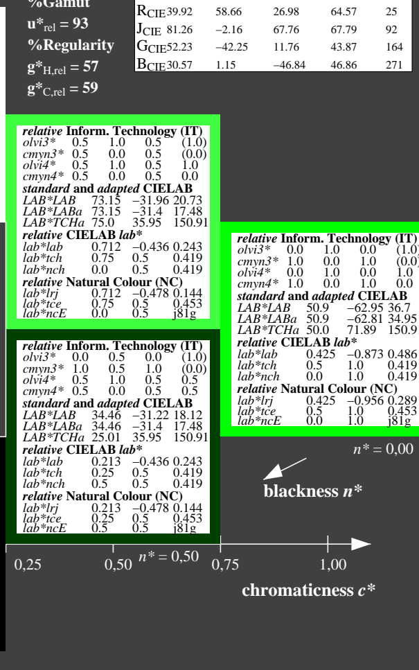
3 step scales for constant CIELAB hue 151/360 = 0.419 (right)
