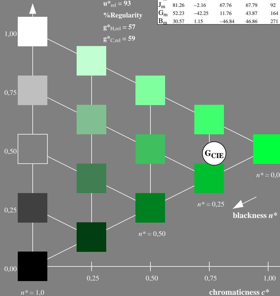
NE220-7, 5 step scales for constant CIE hue 164/360 = 0.457 (left)
