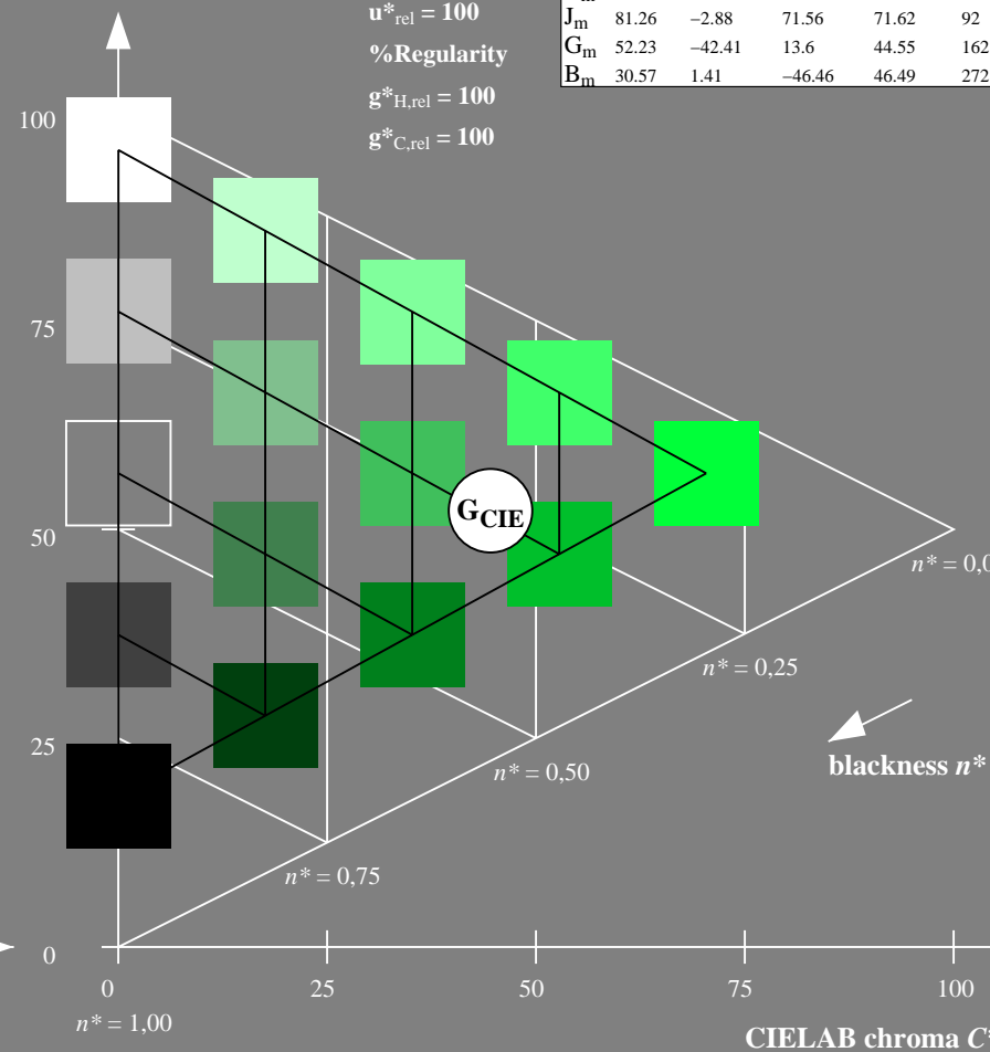
5 step scales for constant CIE hue 162/360 = 0.451 (right)
