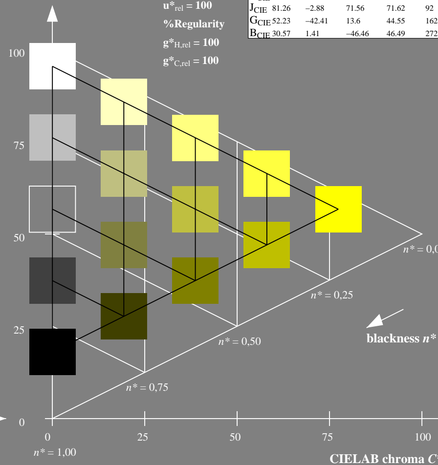
5 step scales for constant CIELAB hue 90/360 = 0.25 (right)
