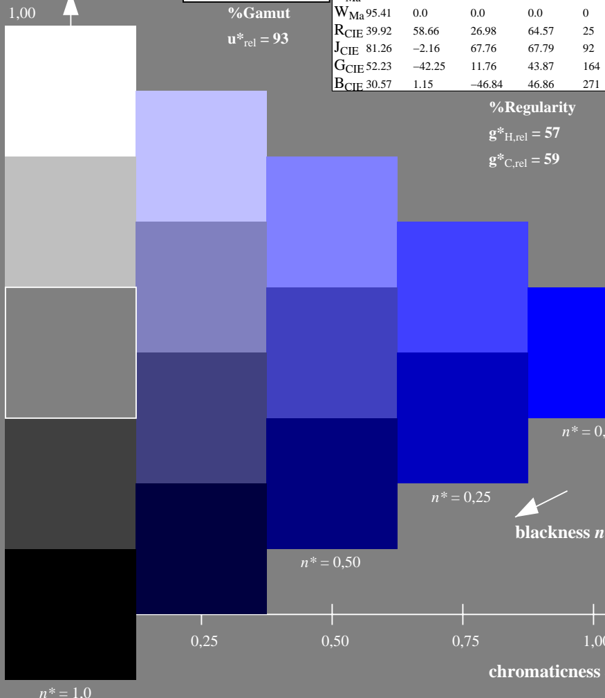
NE40-7, 5 step scales for constant CIELAB hue 305/360 = 0.847 (left)
