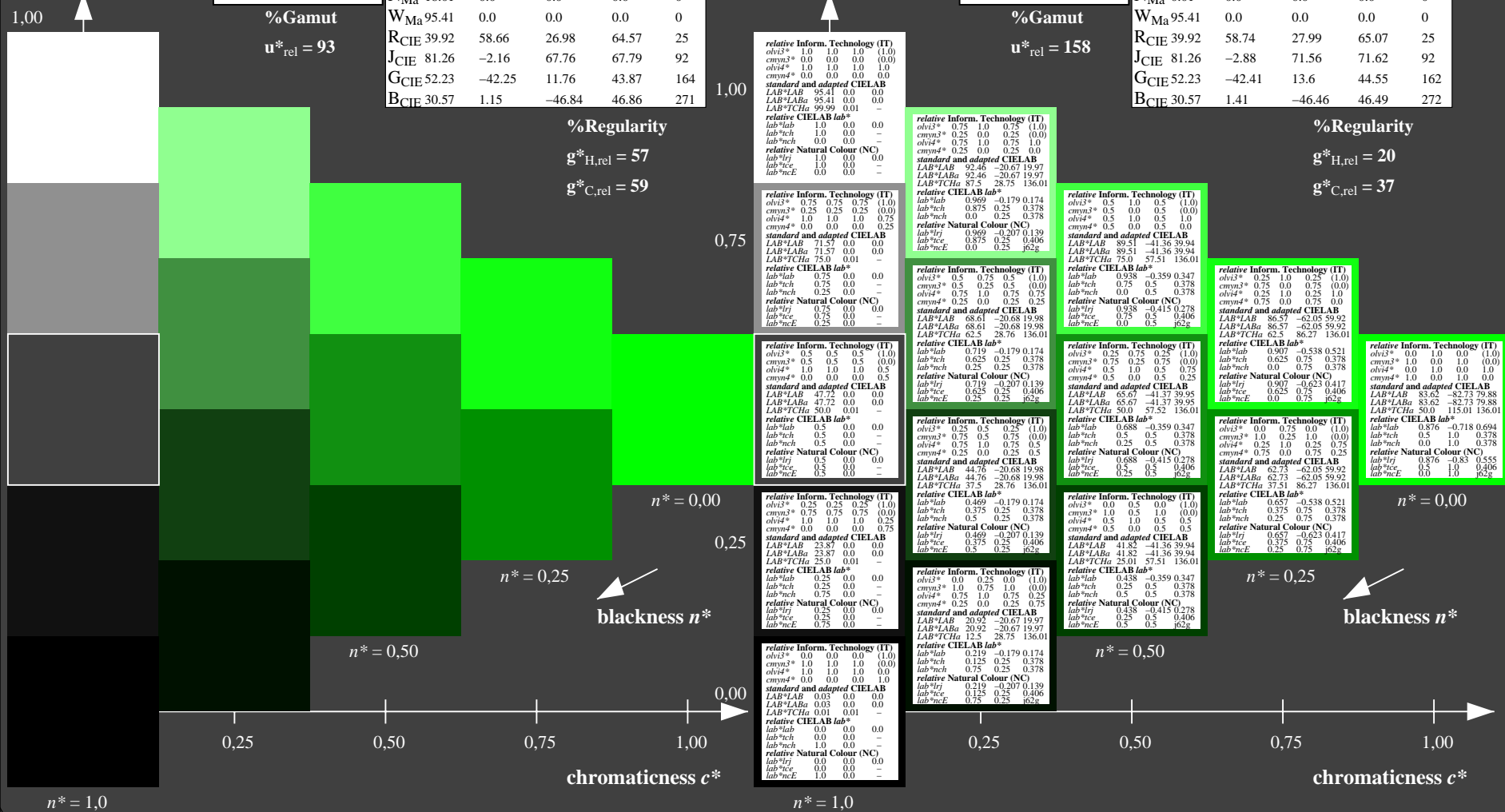
NE400-7, 5 step scales for constant CIELAB hue 151/360 = 0.419 (left)
