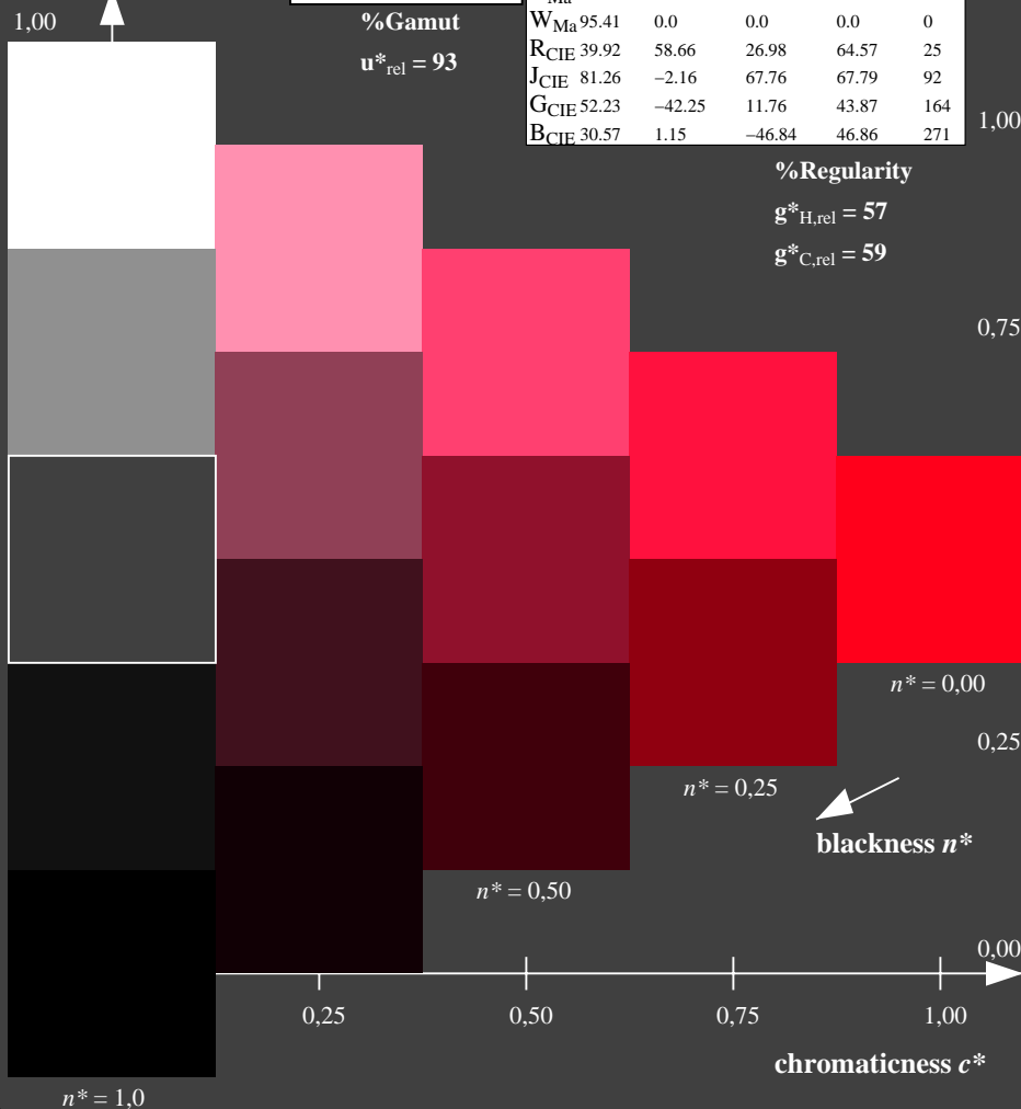
NE40-7, 5 step scales for constant CIELAB hue 25/360 = 0.069 (left)
