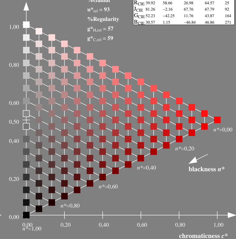
16 step scales for constant CIELAB hue 38/360 = 0.105 (right) input: olv^* setrgbcolor output: no change compared to input
