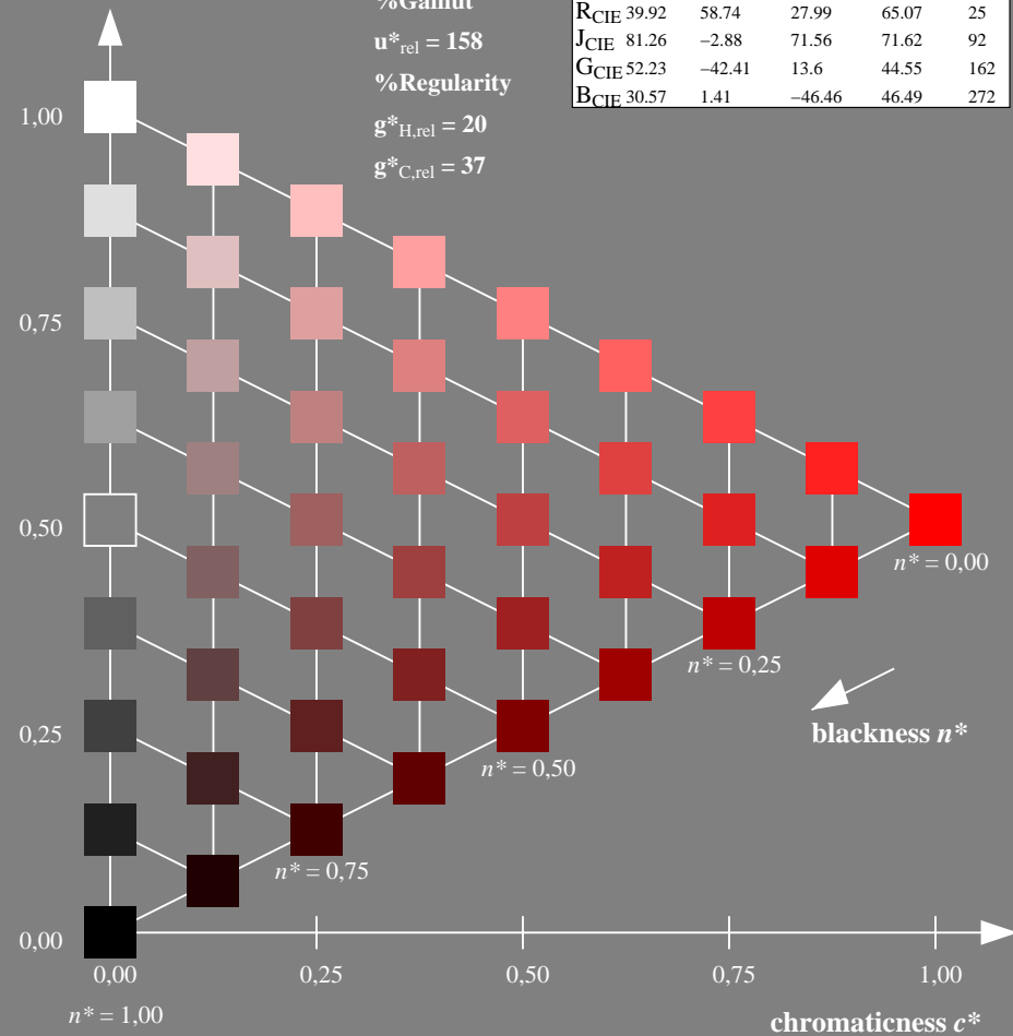
NE750-7, 9 step scales for constant CIELAB hue 40/360 = 0.111 (left) BAM-test chart NE75; Colorimetric systems TLS00 & ORS18 D65: 9 and 16 step colour scales for 10 hues
