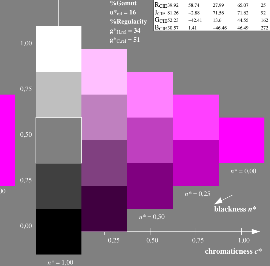
5 step scales for constant CIELAB hue 326/360 = 0.906 (right)
