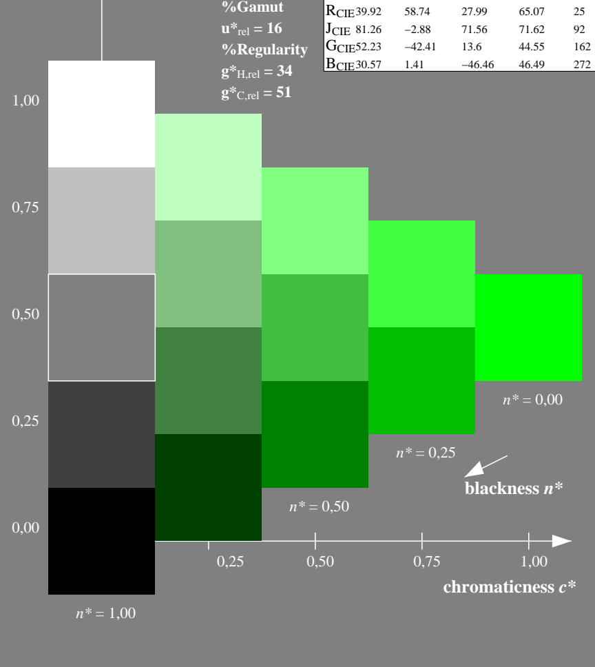
5 step scales for constant CIELAB hue 142/360 = 0.395 (right)
