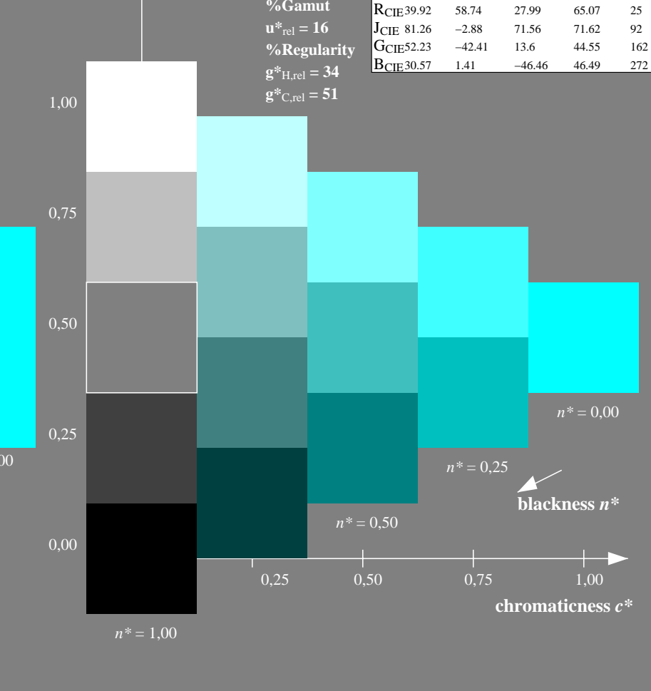
5 step scales for constant CIE LAB hue 198/360 = 0.55 (right)
