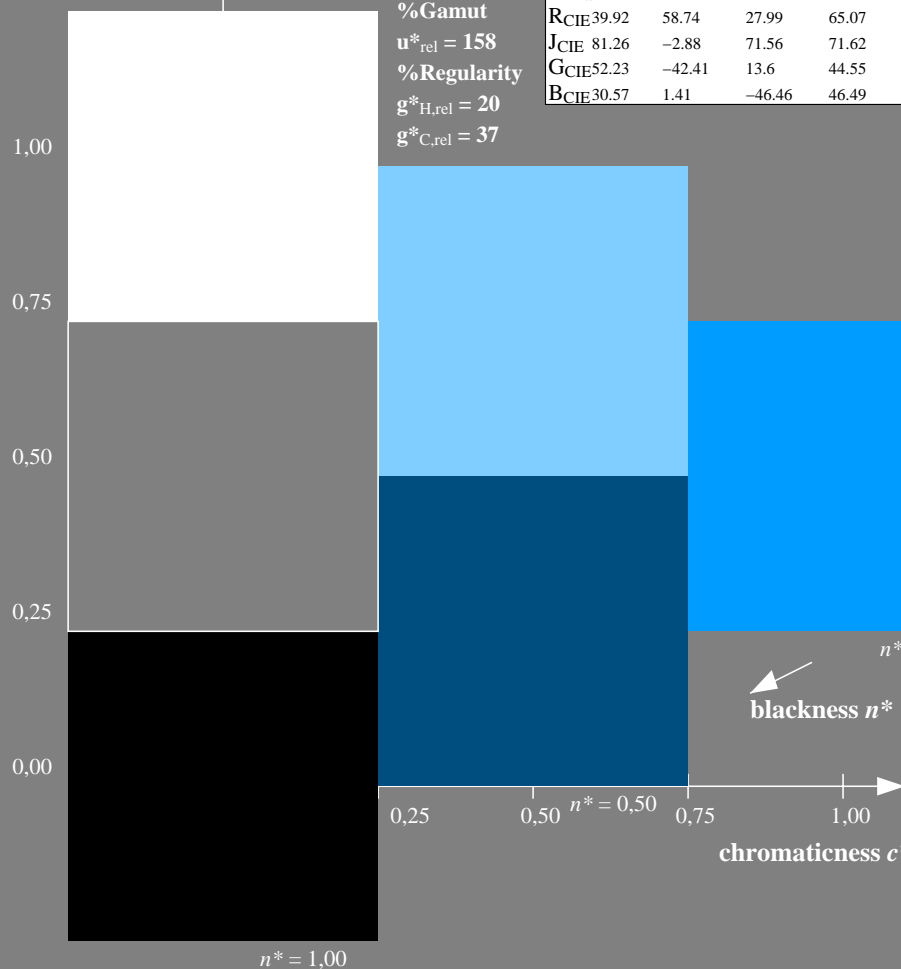
NE830-7, 3 step scales for constant CIELAB hue 272/360 = 0.755 (left)
