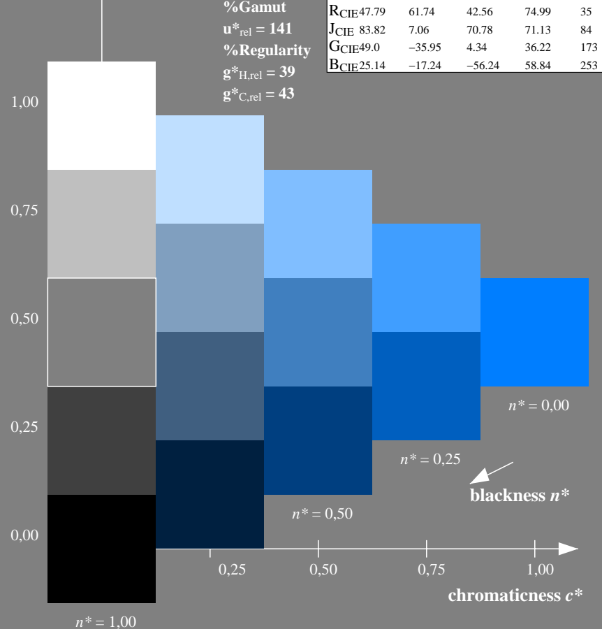
5 step scales for constant CIE LAB hue 253/360 = 0.703 (right)
