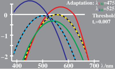
WE060-3, Change of LMS in colour vision; Adaptation
