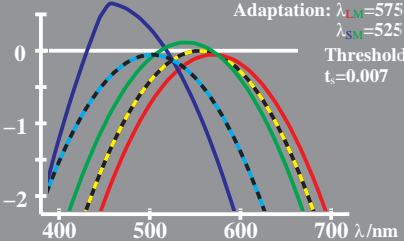
WE060-5, Change of LMS in colour vision; Adaptation
