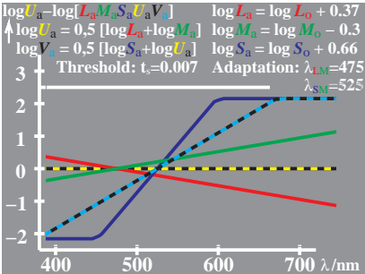
WE061-8, Change of LMS in colour vision; Adaptation
