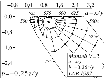
WE511-3, Colours in (a,b) chromaticity diagram
