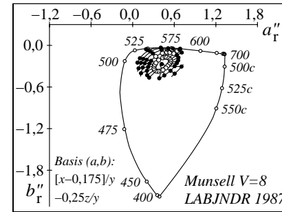
WE531-8, Colours in (a''r,b''r) colour diagram
