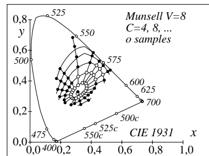
WE530-1, Colours in (x,y) chromaticity diagram
