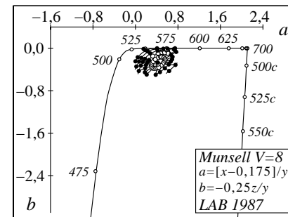
WE531-4, Colours in (a,b) chromaticity diagram
