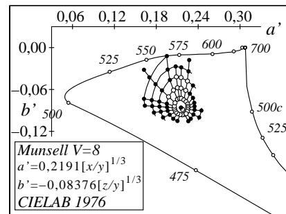
WE530-3, Colours in (a',b') colour diagram
