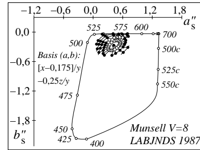
WE531-7, Colours in (a''s,b''s) colour diagram
