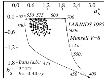
WE530-7, Colours in (a''s,b''s) colour diagram
