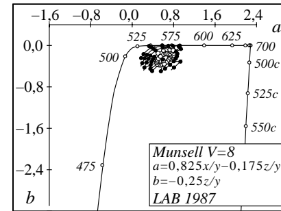
WE531-6, Colours in (a,b) chromaticity diagram
