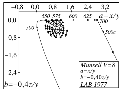
WE530-2, Colours in (a,b) chromaticity diagram
