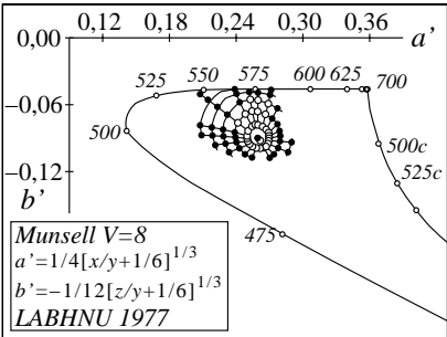
WE530-4, Colours in (a', b') colour diagram
