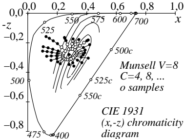
WE531-1, Colours in (x, -z) chromaticity diagram
