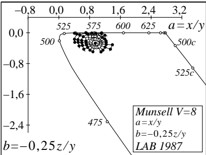
WE531-3, Colours in (a,b) chromaticity diagram
