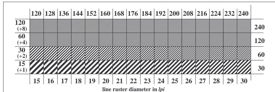
XE781-3, Picture C5: Line raster under 45 (or 135); PS operator: nnn0* setcmymcolor
