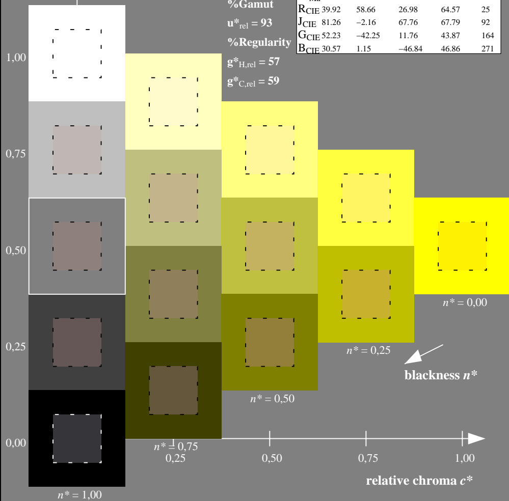
De140-7N, 5 step scales for constant CIELAB hue 96/360 = 0.268 (left)
