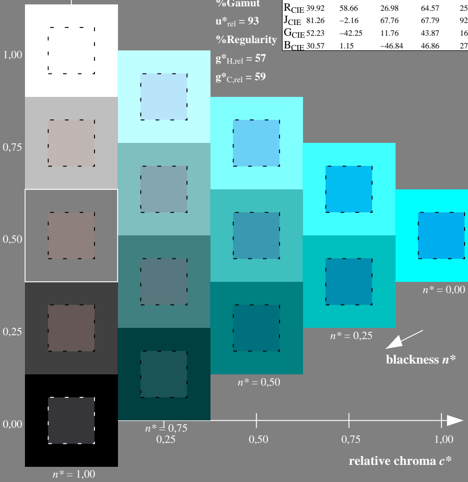
De140-7N, 5 step scales for constant CIELAB hue 236/360 = 0.656 (left)
