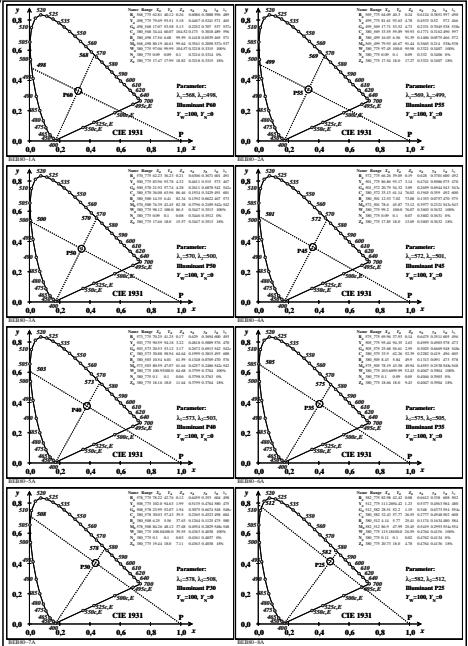
TUB-test chart BEB8; 6 Ostwald optimal colours for 8 illuminants Pxx input: rgb/cmy0/000k/n (left) and Dxx (right), (x, y)400,700, lines separate wavelength ranges of Ostwald optimal colours
