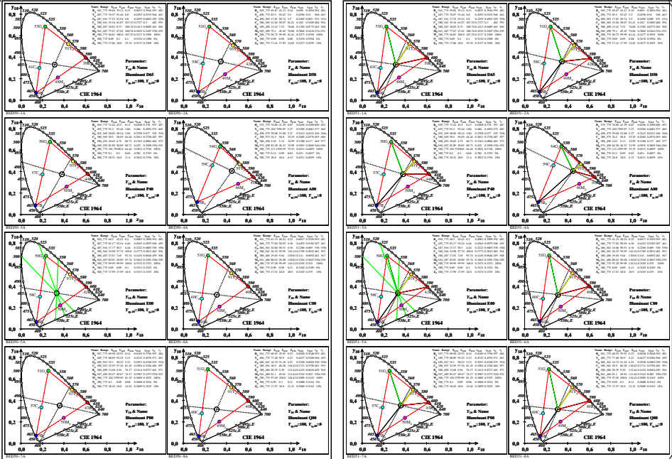
TUB-test chart BED5; 6 Ostwald optimal colours for 8 illuminants Dxx, input: rgb/cmy0/000k/n CIE-10, diagrams (x10, y10), C>288:1
