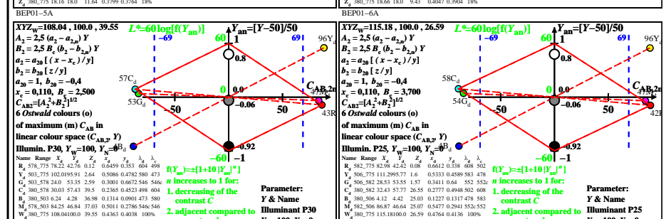
TUB-test chart BEP0; 6 Ostwald optimal colours for 8 illuminants Pxx, input: rgb/cmy0/000k/n CIE-02, diagrams ( C_{AB,2}, Y ), C>288:1 , scale Y=-1 to 1 , antagonic reflection
