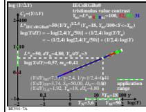
TUB-test chart BEVO; IECsRGB0, L^* & L^* for Y/Y_u with additional data, Y_{nc} = (Y & L^*)/Y_{nc} Absolute and relative lightness, sensitivity and contrast, S_{90} = 50.00, 1/\gamma = 1/2.4 = 0.41
