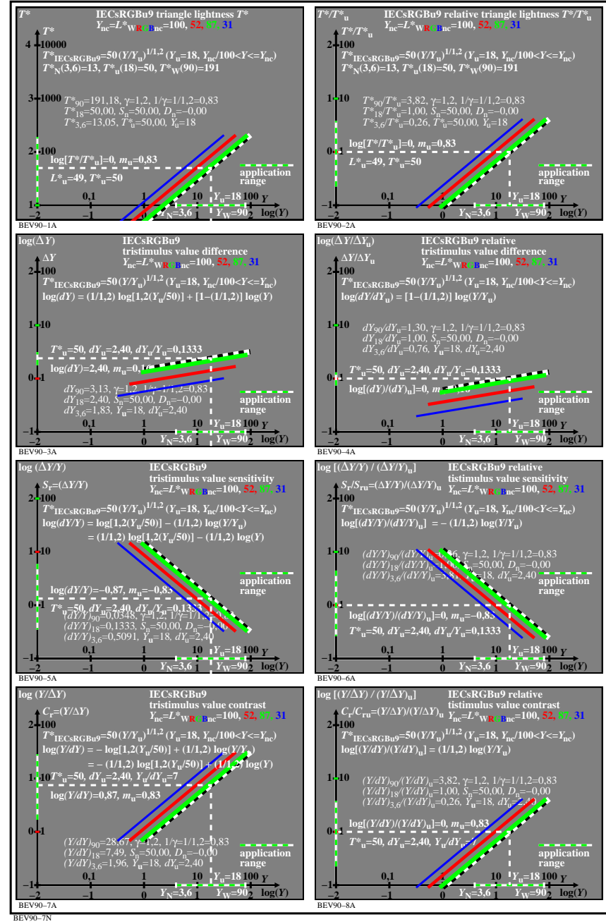
TUB-test chart BEV9; IECsRGBu9, t^* & T^* for Y/Y_u with additional data, Y_{nc}=(Y \& L^*)WRGB_{nc} Absolute and relative lightness, sensitivity and contrast, S_n=50,00 , 1/\gamma=1/1,2=0,83
