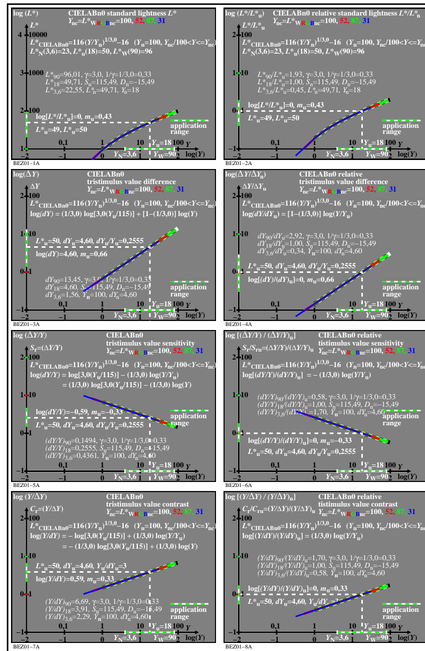
TUB-test chart BEZO; CIELABn0, l^* & L^* for Y/Y_n with additional data, Y_{nc}=(Y \cdot L^*)W_{nc} Absolute and relative lightness, sensitivity and contrast, S_n=115,49 , 1/\gamma=1/3,0=0,33 , D_n=-15,49
