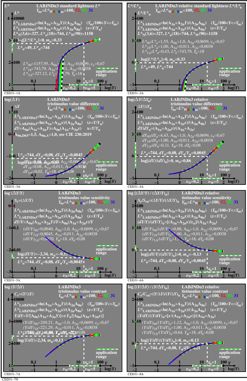
TUB-test chart CED3; LABJNDu3, I^*(Y) & L^*(Y) , Y_{nc}=(Y \cdot L^*)_{W_{nc}} , c_X=0,66 , with more data Absolute and relative lightness, sensitivity and contrast, A_{0n}=1,5 , A_{1n}=0,011 , A_{2n}=0,0038 , A_{2u}=0,068
