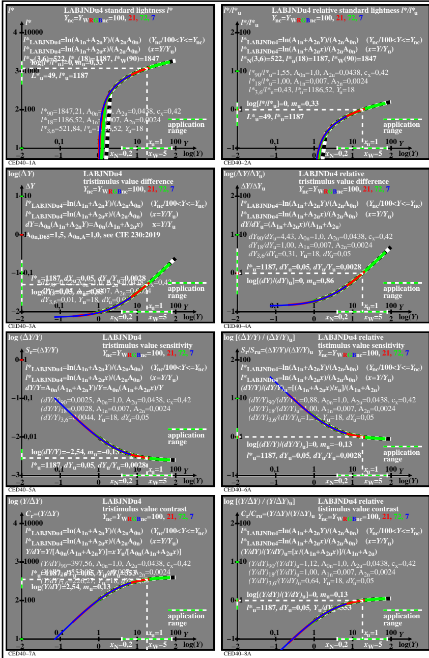
TUB-test chart CED4; LABJNDu4, l^*(Y) & L^*(Y) , Y_{nc} = (Y \cdot L^*)_{W_{nc}} , c_x = 0.43 , with more data Absolute and relative lightness, sensitivity and contrast, A_{0n} = 1.5, A_{1n} = 0.007, A_{2n} = 0.0024, A_{2u} = 0.044
