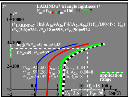
CED70-1A
