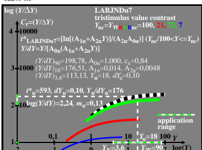
CED70-7A
