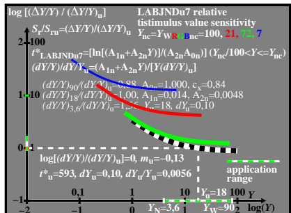
CED70-6A
