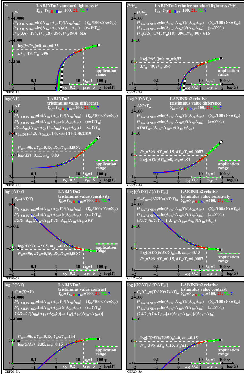
TUB-test chart CEF2; LABJNDu2, l^*(Y) & L^*(Y) , Y_{nc}=(Y \cdot L^*)_{Wnc} ; c_x=0,86 Absolute and relative lightness, sensitivity and contrast, A_{0n}=1,5, A_{1n}=0,017, A_{2n}=0,0049, A_{2u}=0,089
