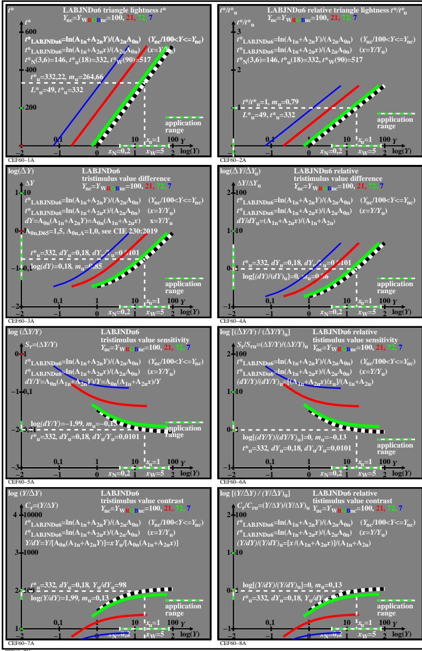
TUB-test chart CEF6; LABJNDu6, t^*(Y) & T^*(Y) , Y_{nc}=(Y \cdot L^*)WR_{RGBnc} , c_x=1,00 Absolute and relative lightness, sensitivity and contrast, A_{0n}=1,5, A_{1n}=0,017, A_{2n}=0,0058, A_{2u}=0,104
