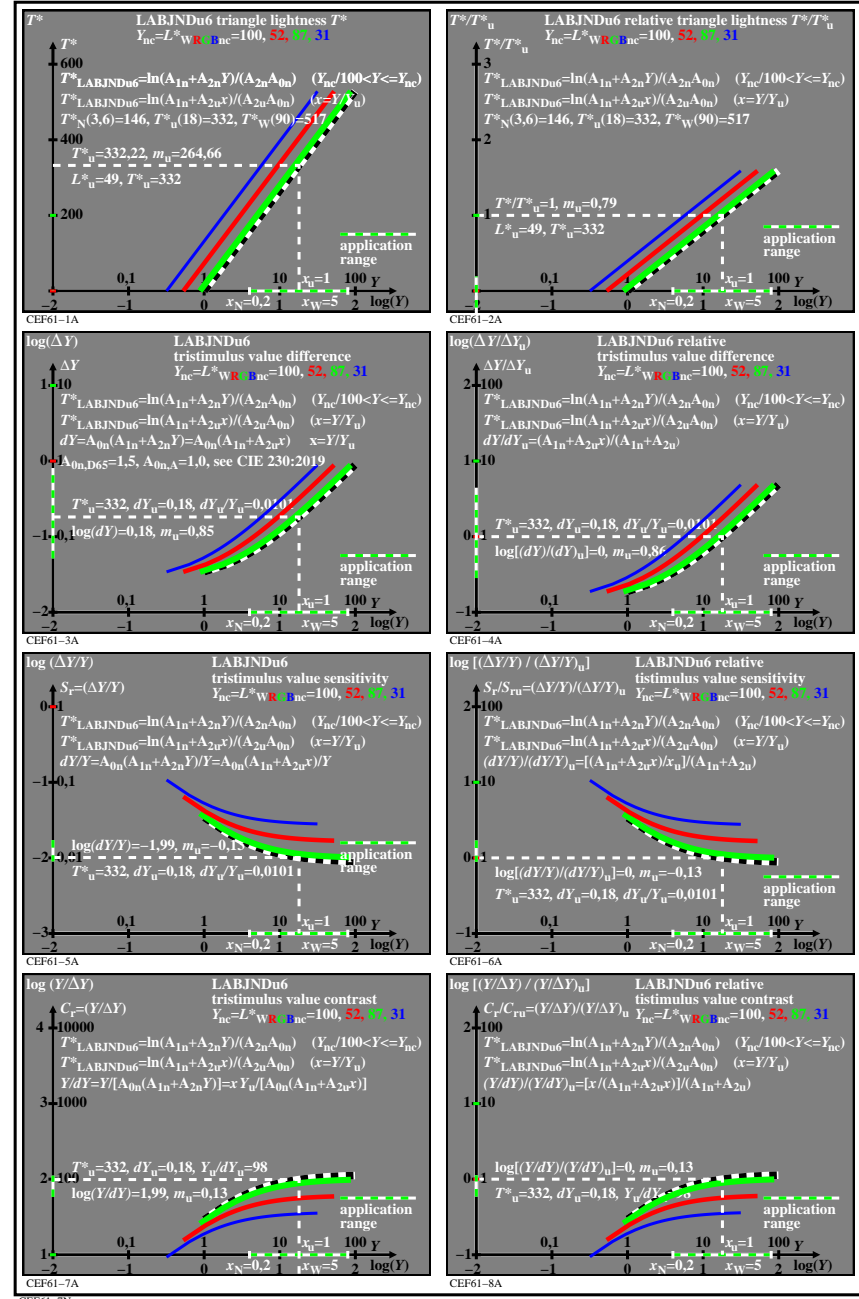
TUB-test chart CEF6; LABJNDu6, t^*(Y) & T^*(Y) , Y_{nc}=(Y \cdot L^*)WR_{RGBnc} , c_x=1,00 Absolute and relative lightness, sensitivity and contrast, A_{0n}=1,5, A_{1n}=0,017, A_{2n}=0,0058, A_{2u}=0,104
