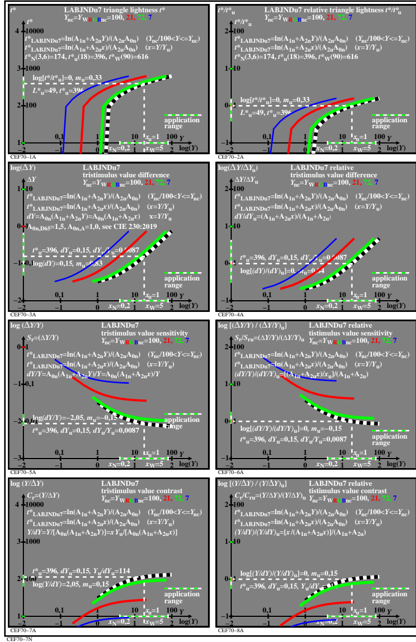
TUB-test chart CEF7; LABJNDu7, t^*(Y) & T^*(Y) , Y_{nc}=(Y \cdot L^*)_{WRGBnc} , c_x=0,86 Absolute and relative lightness, sensitivity and contrast, A_{0n}=1,5, A_{1n}=0,017, A_{2n}=0,0049, A_{2u}=0,089
