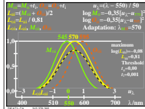
TUB-test chart DEA7; Relative colour vision: 495(C), 520(G), 545-557-570(MVL), 595(O) log & lin [Sensitivities and excitations] LMS-R21\_M_x ( x=1,2,3,4 ); threshold t_0=0,00 and t_1=0,001
