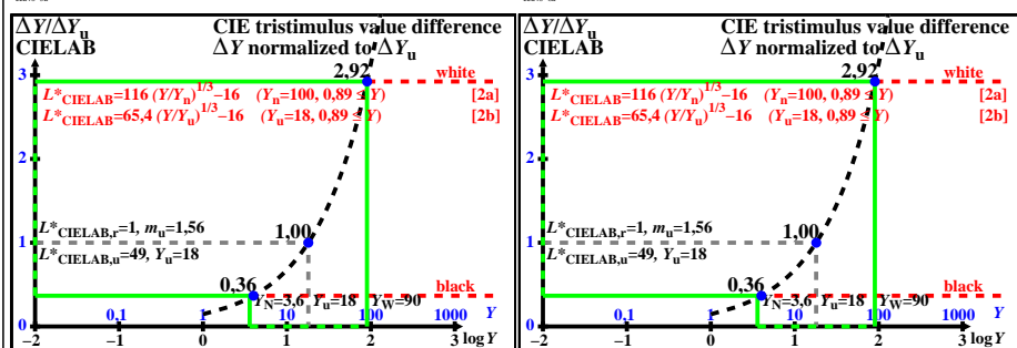
TUB-test chart eea4; Colourimetric data L^*/L_u^*, \Delta Y/\Delta Y_u, (\Delta Y/Y)/(\Delta Y_u/Y_u), (Y/\Delta Y)/(Y_u/\Delta Y_u) = f[\log(Y)] of colour space CIE LAB, see ISO/CIE 11664-4
