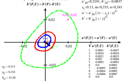
Munsell (Retnotation) Chroma C = 2 and Value V = 1, 5, and 9 in chromaticity diagram ( a'(F,U) , b'(F,U) )
