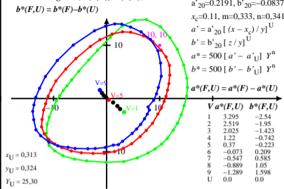
Munsell (Retnotation) Chroma C = 2 and Value V = 1, 5, and 9 in chroma diagram ( a^*(F,U) , b^*(F,U) )
