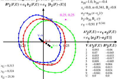
Munsell (Renotation) Chroma C = 2 and Value V = 1, 5, and 9 in chroma diagram ( A_2^*(F,U) , B_2^*(F,U) )
