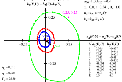
Munsell (Renotation) Chroma C = 2 and Value V = 1, 5, and 9 in chromaticity diagram ( a_2(F,U) , b_2(F,U) )
