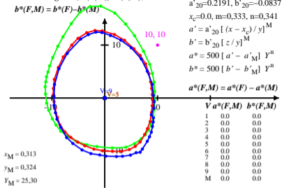
Munsell (Renotation) Chroma C = 2 and Value V = 1, 5, and 9 in chroma diagram ( a^*(F,M) , b^*(F,M) )
