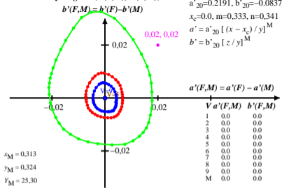
Munsell (Renotation) Chroma C = 2 and Value V = 1, 5, and 9 in chromaticity diagram ( a'(F,M) , b'(F,M) )
