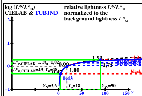
TUB-test chart eee3; Relative lightness \log[L^*/L^*_{u}] = f(Y) of colour spaces CIELAB & TUBJND, see ISO/CIE 11664-4 & CIE 230, many information (left), and less (right)
