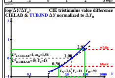
TUB-test chart eee4; CIE tristimulus value difference \log[\Delta Y/\Delta Y_u] = f[\log(Y)] of colour spaces CIELAB & TUBJND; see ISO/CIE 11664-4 & CIE 230, many information (left), and less (right)
