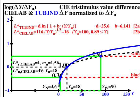
TUB-test chart eee5; CIE tristimulus value difference \log[\Delta Y/\Delta Y_u] = f(Y) of colour spaces CIELAB & TUBJND, see ISO/CIE 11664-4 & CIE 230, many information (left), and less (right)
