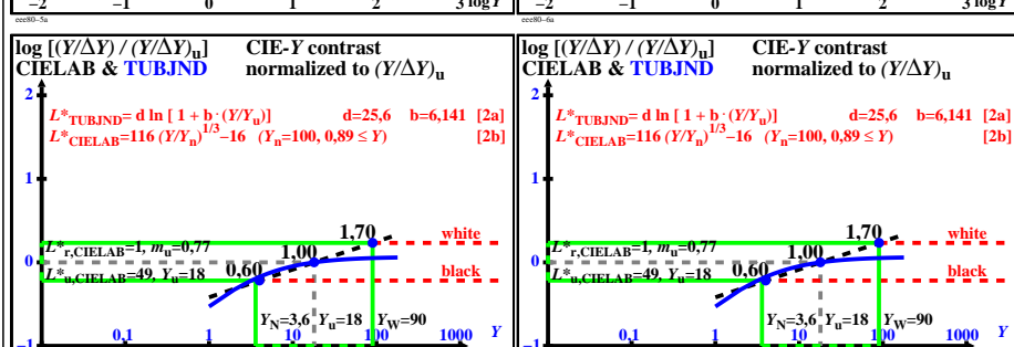
TUB-test chart eee8; Contrast \log [(Y/Delta Y) / (Y/Delta Y)_u] = f[\log(Y)] of colour spaces CIELAB & TUBJND, see ISO/CIE 11664-4 & CIE 230, many information (left), and less (right)
