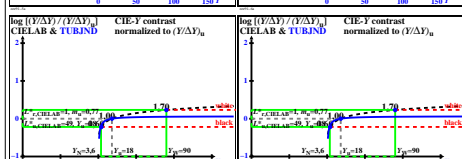
TUB-test chart eee9; Contrast \log \left[ \frac{(Y/DY)}{(Y/DY)_u} \right] = f(Y) of colour spaces CIELAB & TUBJND, see ISO/CIE 11664-4 & CIE 230, many information (left), and less (right)
