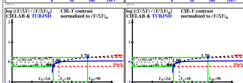
TUB-test chart eee9; Contrast \log [(Y/\Delta Y) / (Y/\Delta Y)_u] = f(Y) of colour spaces CIELAB & TUBJND, see ISO/CIE 11664-4 & CIE 230, many information (left), and less (right)
