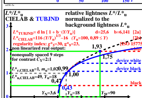
TUB-test chart eef3; Relative lightness L^*/L_u^* = f(Y) of colour spaces CIELAB & TUBJND, see ISO/CIE 11664-4 & CIE 230, many information (left), and less (right)
