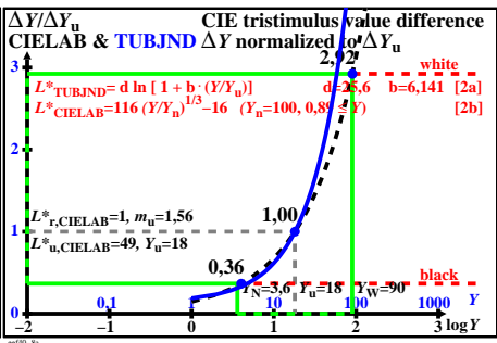
TUB-test chart eef4; CIE tristimulus value difference \Delta Y/\Delta Y_u = f[\log(Y)] of colour spaces CIELAB & TUBJND, see ISO/CIE 11664-4 & CIE 230, many information (left), and less (right)
