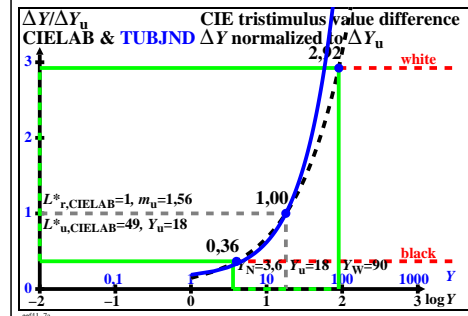
TUB-test chart eef4; CIE tristimulus value difference \Delta Y/\Delta Y_u = f[\log(Y)] of colour spaces CIELAB & TUBJND, see ISO/CIE 11664-4 & CIE 230, many information (left), and less (right)
