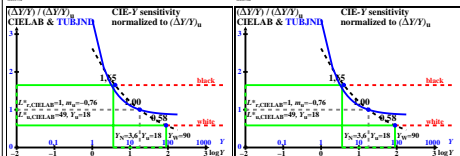
TUB-test chart eef6: Sensitivity (\Delta Y/Y) / (\Delta Y/Y)_u = f[\log(Y)] of colour spaces CIELAB & TUBJND, see ISO/CIE 11664-4 and CIE 230, many information (left), and less (right)
