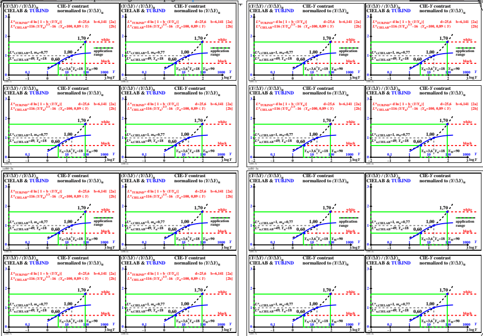
TUB-test chart eef8; Contrast (Y/\Delta Y) / (Y/\Delta Y)_0 = f[\log(Y)] of colour spaces CIELAB & TUBJND, see ISO/CIE 11664-4 & CIE 230, many information (left), and less (right)
