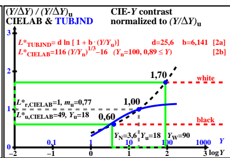
TUB-test chart eef8; Contrast (Y/\Delta Y) / (Y/\Delta Y)_u = f[\log(Y)] of colour spaces CIELAB & TUBJND, see ISO/CIE 11664-4 & CIE 230, many information (left), and less (right)
