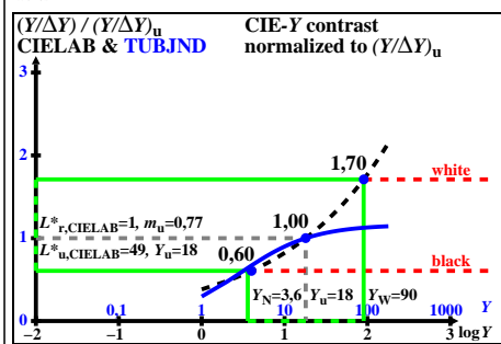
TUB-test chart eef8; Contrast (Y/\Delta Y) / (Y/\Delta Y)_u = f[\log(Y)] of colour spaces CIELAB & TUBJND, see ISO/CIE 11664-4 & CIE 230, many information (left), and less (right)
