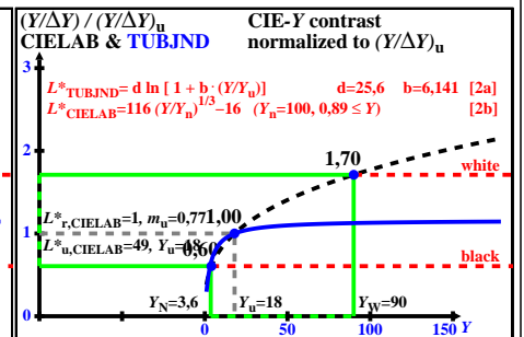
TUB-test chart eef9; Contrast (Y/\Delta Y) / (Y/\Delta Y)_u = f(Y) of colour spaces CIELAB & TUBJND, see ISO/CIE 11664-4 & CIE 230, many information (left), and less (right)
